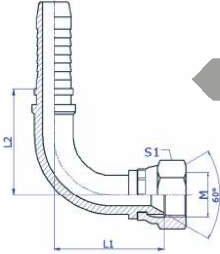
METRİK SOMUNLU 60° HAVŞALI 90° HORTUM REKORU METRIC 90° FEMALE - 60° "KOMATSU" CONE SEAT
