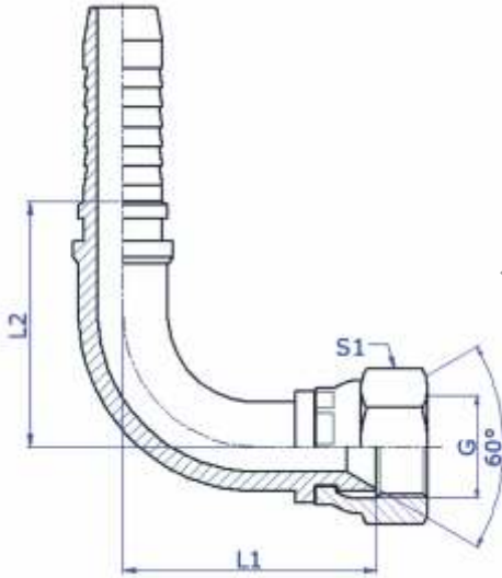
BSP SOMUNLU 60° HAVŞALI 90° HORTUM REKORU BSP 90° FEMALE - 60° CONE SEAT
